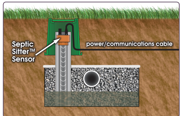
Traditional stone trench installation
