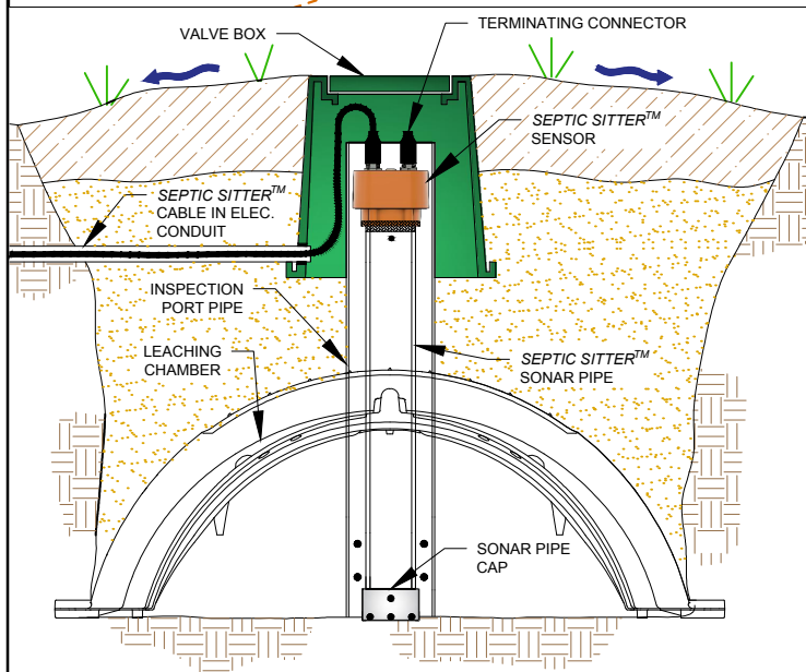
CROSS SECTION SHOWING SEPTIC SITTER™ SENSOR WITH TERMINATING CONNECTOR
